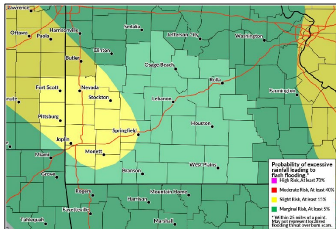
Excessive Rainfall Outlook (Tonight - Tuesday Morning)
