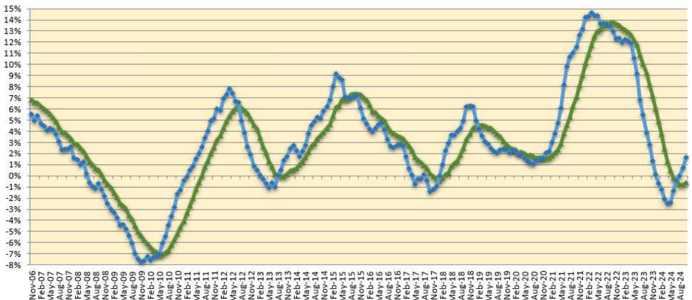
General Fund Sales Tax Trend 12 Month Rolling Average of 1yr Avg Growth of the 3 & 12 Month Rolling Average of Sales Tax Receipts
