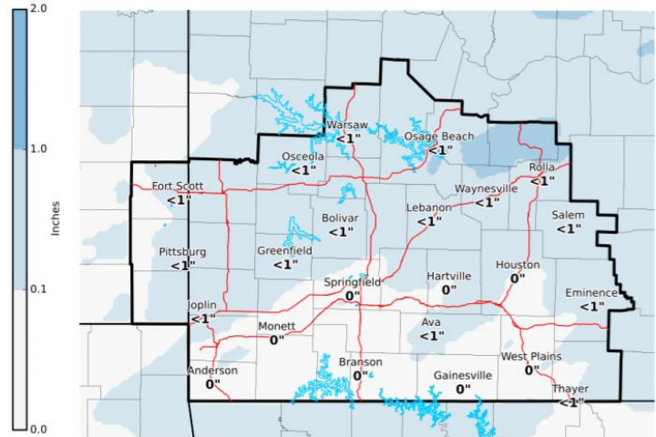
Expected Snowfall - Official NWS Forecast Valid: 11/11/2019 12:00 AM - 11/11/2019 06:00 PM CST
