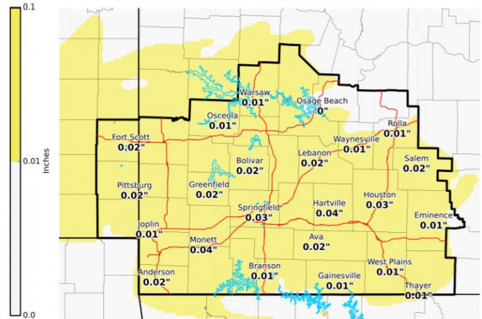
Expected Ice Accumulation - Official NWS Forecast Valid: 11/11/2019 12:00 AM - 11/11/2019 06:00 PM CST
