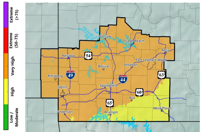
Grassland Fire Danger Index (GFDI) Valid: 02/18/2018 11:00 AM - 02/19/2018 06:00 AM CST
